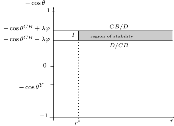
Figure 10: Stable Cassie–Baxter drops with untrahydrophobic contact angles on a dry hydrophilic surface
