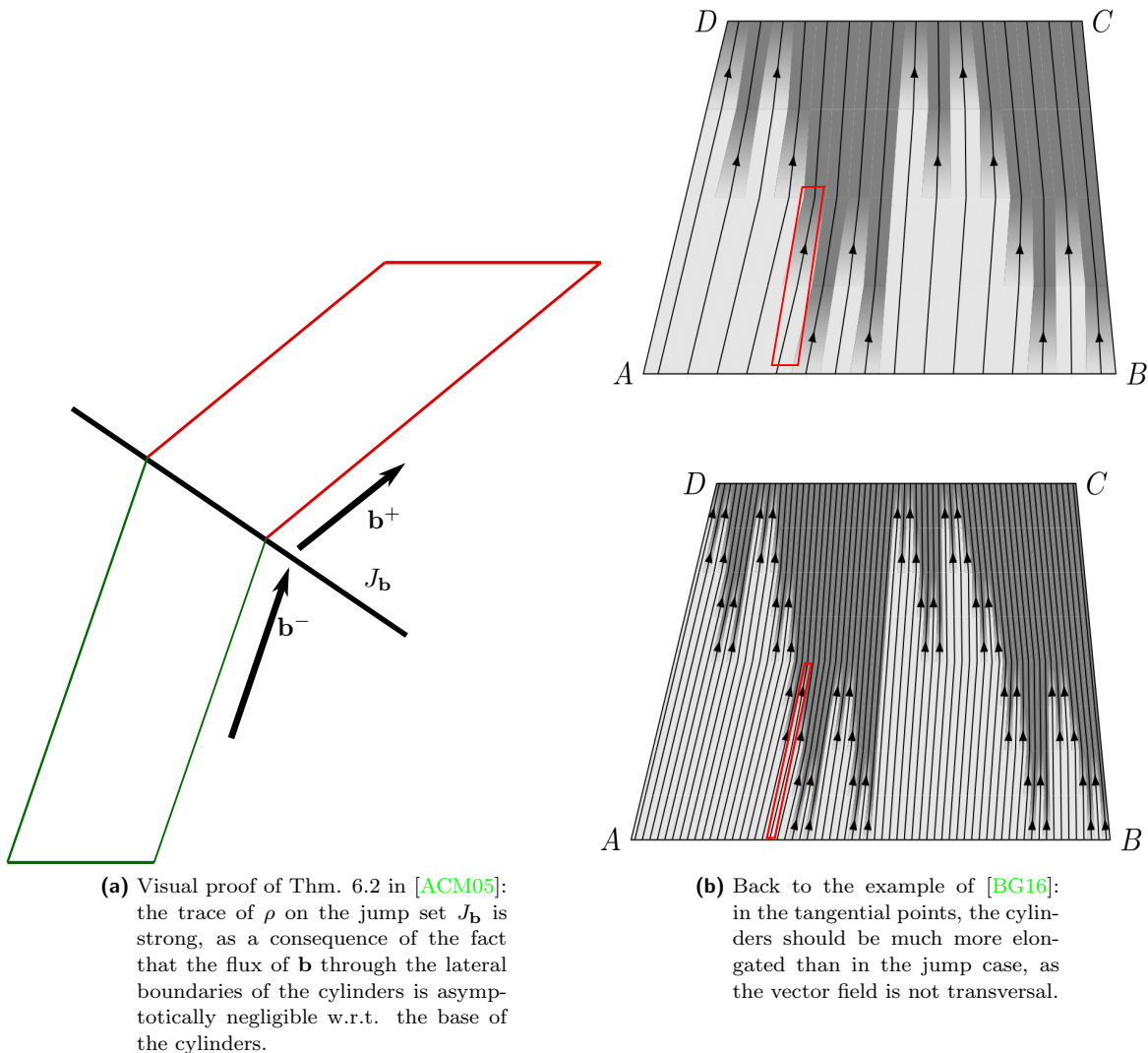
Figure 2. Strong traces via cylinders: the jump case vs the Cantor case.
