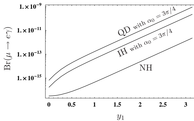
FIG. 4: The LFV branching ratios \text{Br}(\mu \rightarrow e\gamma) are shown in the NH case, the IH case with \alpha_0 = 3\pi/4 and the QD case with \alpha_0 = 3\pi/4 for R = OQ_1 .
