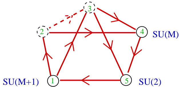
Figure 7: Quiver of the dP_3 theory for generic M and P = K = 1 . The dashed nodes represent “ SU(1) ” factors while the dashed line a bi-fundamental field which completely decouples in the IR and plays no rôle. This theory is essentially the same as the one for dP_2 , see Figure 5.
