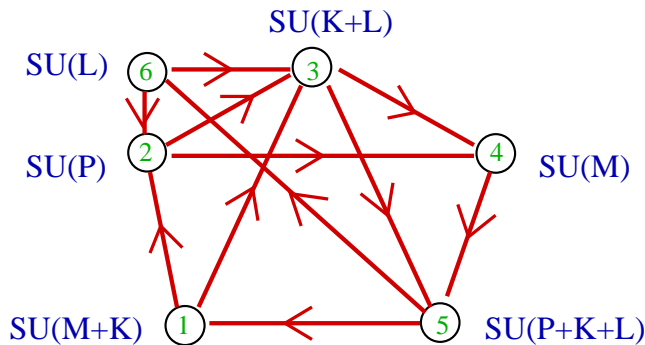
Figure 8: Quiver of the PdP_4 theory for generic M, P, K and L .
