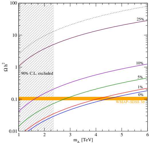
Figure 2: Relic density versus the A_-^{(1)} mass, for a few values of the relative mass splitting between A_-^{(1)} and b_-^{(1)} , and in the case of the g_+^{(2)} on resonance in b_-^{(1)} pair annihilations.
