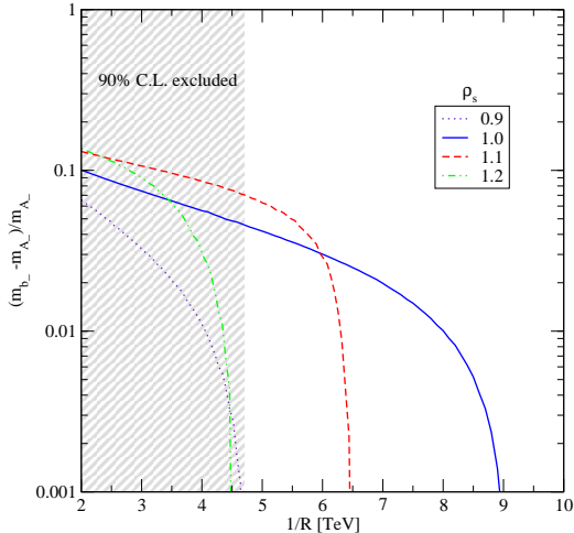
Figure 5: Correlation between the A_-^{(1)} - b_-^{(1)} mass splitting and compactification radius in models with \Omega h^2 matching the best fit value from cosmological observations, for a few values of \rho_s .
