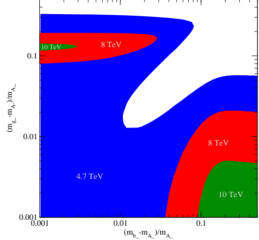
Figure 9: For a few selected values of the compactification scale, regions in the parameter space m_{g_-}^{(1)} - m_{A_-}^{(1)} versus m_{b_-}^{(1)} - m_{A_-}^{(1)} in which \Omega h^2 is lower or equal to the best fit value from cosmological observations.
