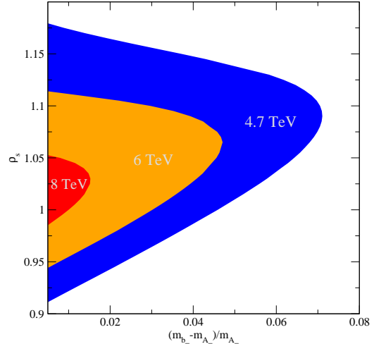
Figure 6: For a few selected values of the compactification scale, regions in the parameter space \rho_s -mass splitting in which \Omega h^2 is lower or equal to the best fit value from cosmological observations.
