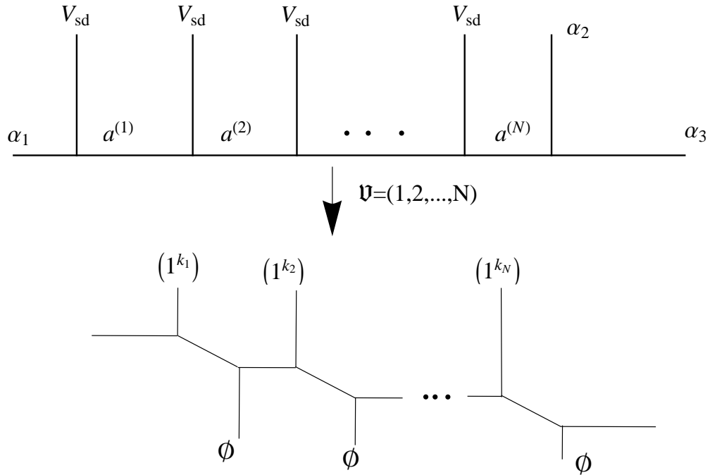
Figure 8: relation between SU(N) vortex and CFT
