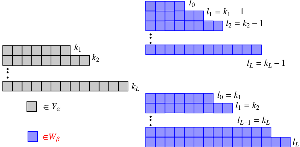
Figure 11: Relation between Y_\alpha and W_\beta when m_{\alpha,\beta} = \epsilon_2
