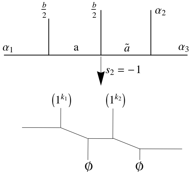
Figure 4: relation between SU(2) vortex and CFT
