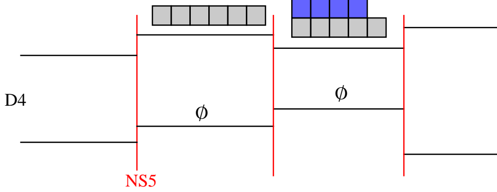
Figure 3: SU(2) simple surface operators from quiver theory
