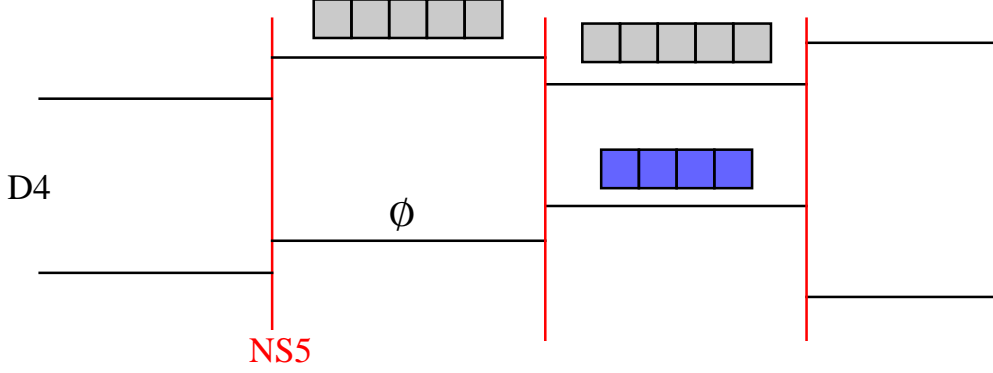
Figure 2: SU(2) vortex from quiver theory
