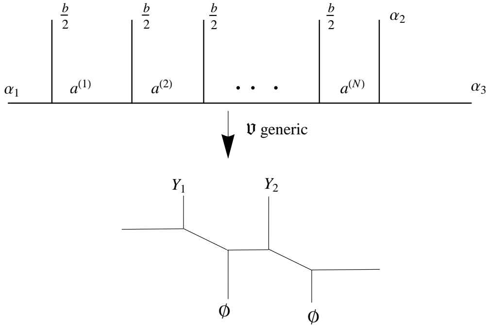
Figure 6: relation between SU(2) strip amplitudes and CFT
